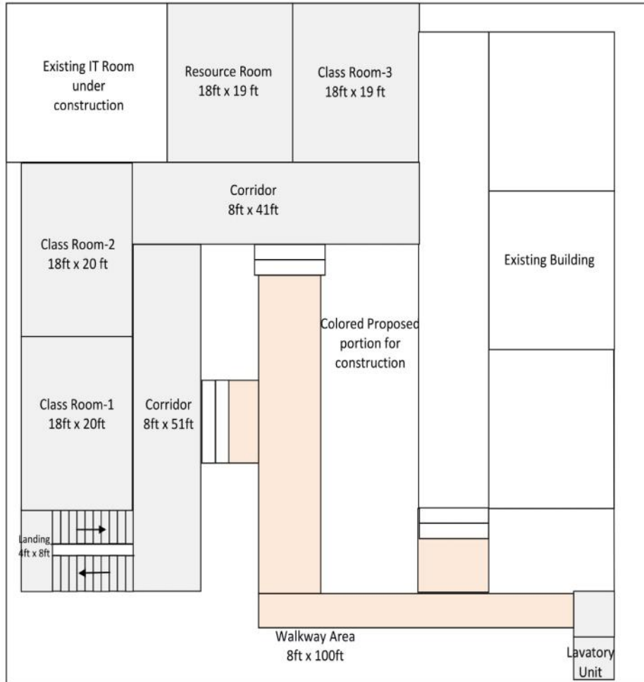
Plan of Madni Elementary School Supported by SEF/UEP District Matyari
