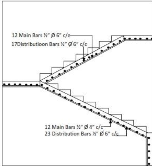
Section of Stair Case
