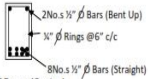
Roof Beam (Center) 9" x 18"
